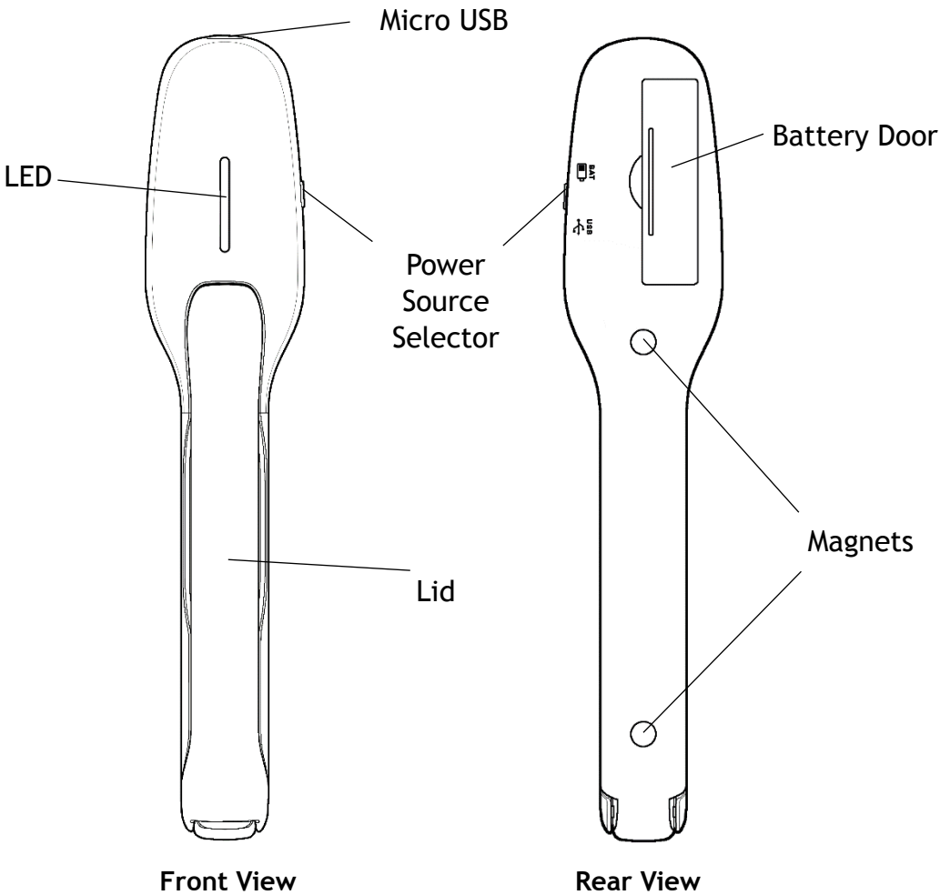
Figure 22. Front and Rear views of Smart Repeater (SR200)
