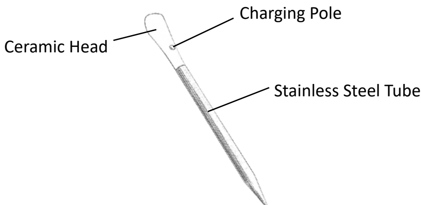
Figure 1. Intelligent Wireless Food Thermometer (ECPIN)
